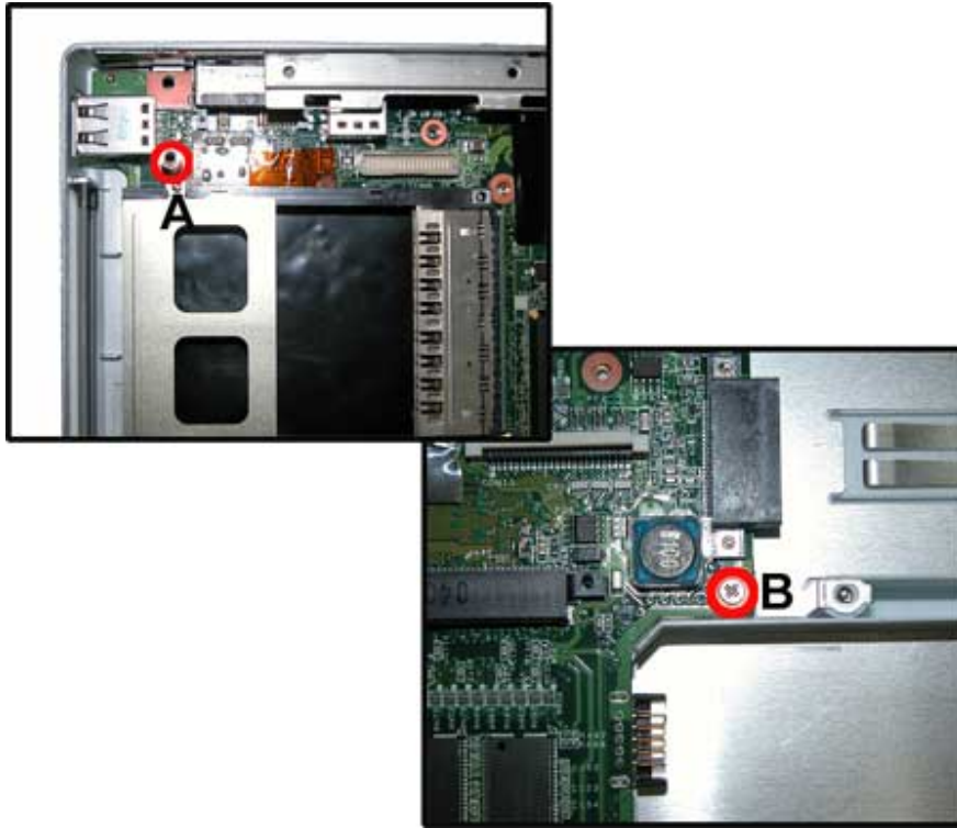
Fig. 32 Screws on Main Board
